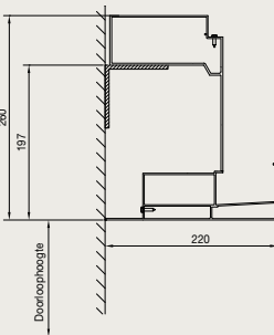
Pivot Façade-mounted
