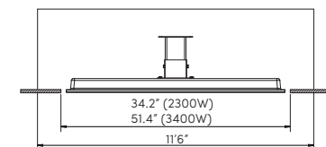
MINIMUM CAVITY OPTION 2
