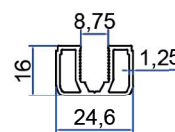
8mm glass adaptor profile
