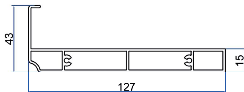
Bottom Base profile
