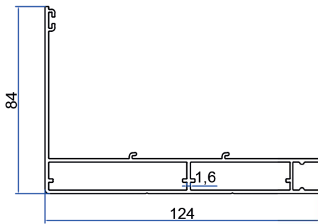
Runner profile
