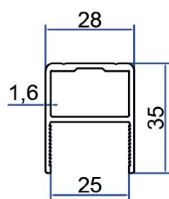
Top & Bottom glass profile
