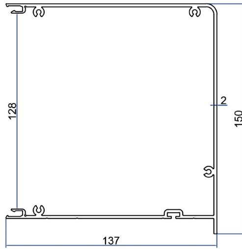
Motor Box profile
