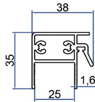
Intermediate glass profile
