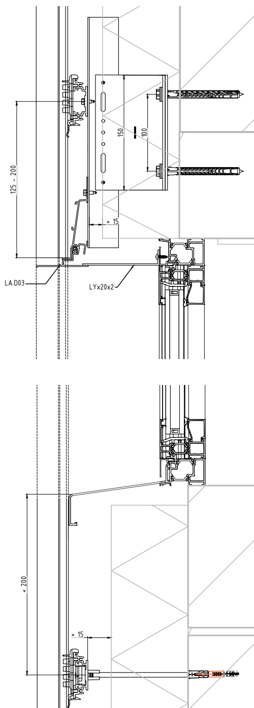
Direct fixation
