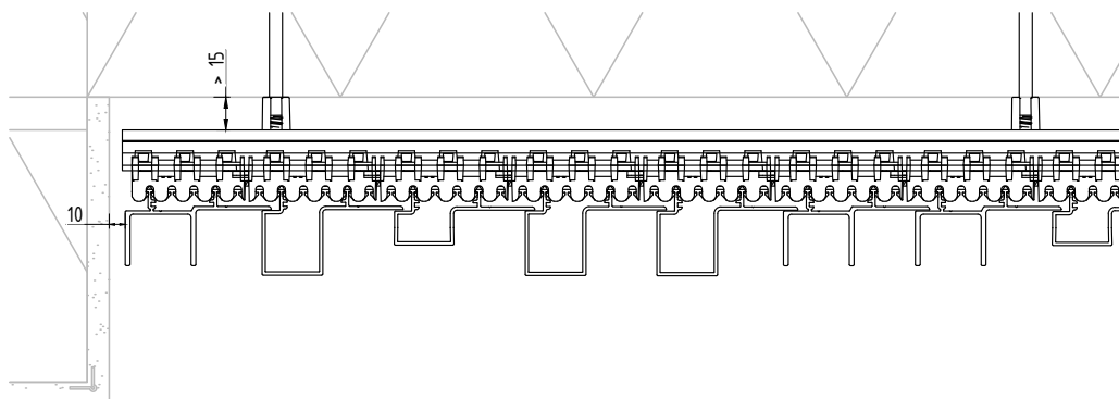
Direct fixation
