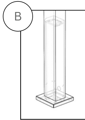
24 inch recessed column base with 9" square floor mounting plate.
