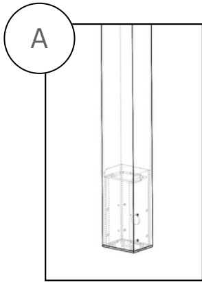
16 inch recessed column base.
