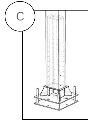
Adjustable steel sleeves.
