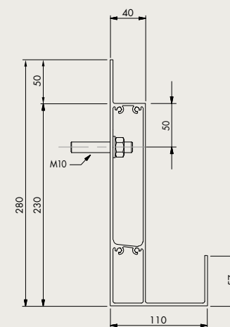
Span and Pivot, with wall connection profile
