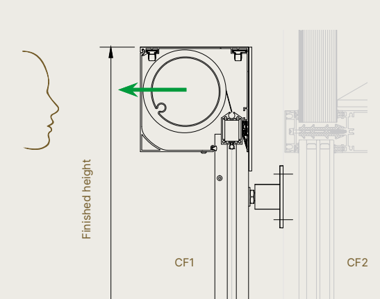
Fixscreen® 150 - Drawing surface-mounted curtain wall
