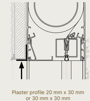
Plaster profile
