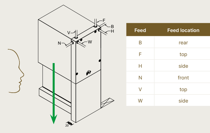
Cable feed
