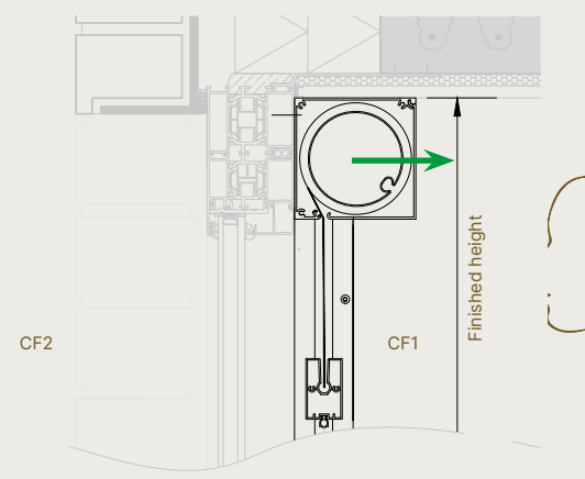
Fixscreen® 100 - Drawing surface-mounted indoor application
