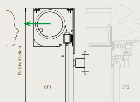
Fixscreen® 150 - Drawing surface-mounted masonry
