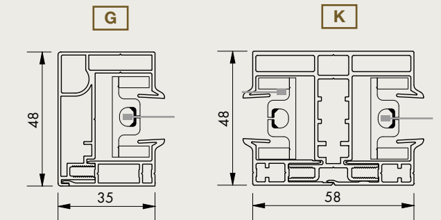
Side guiding channels
