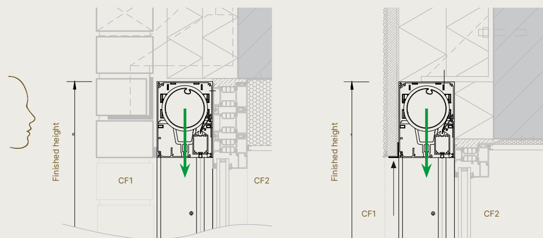
Drawing surface-mounted masonry
