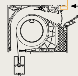
Finishing profile (option)
