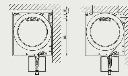
Hook profile
