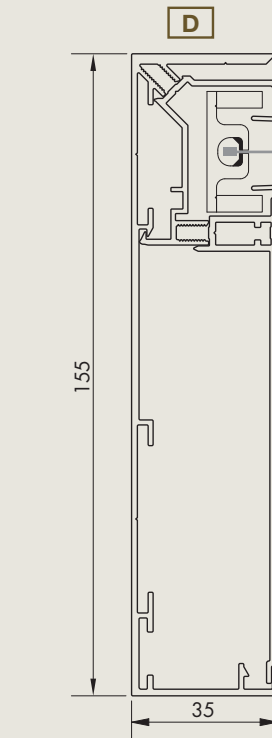
D = deep side guiding channel (standard)
