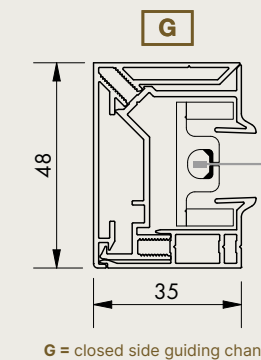
Side guiding channels
