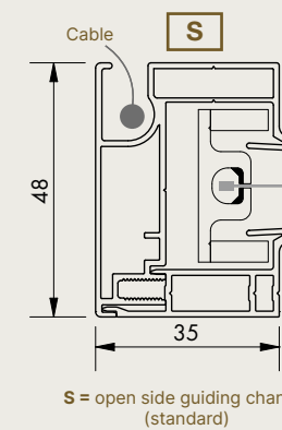
Side guiding channels
