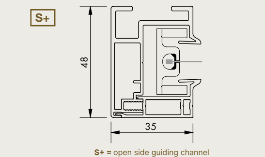
Side guiding channel
