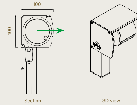
Fixscreen® 100 - Head box
