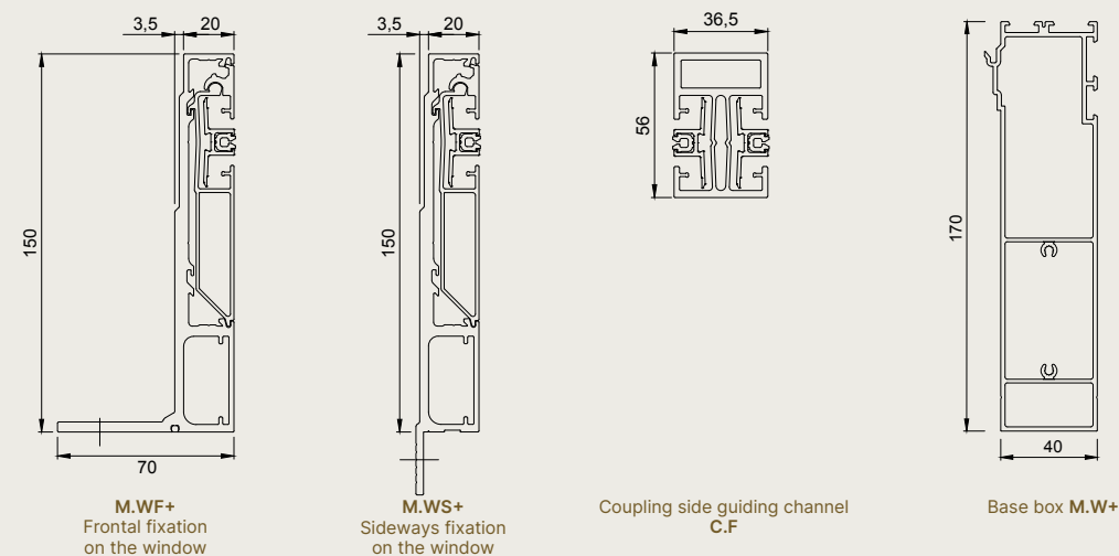
Installation with 40 mm filler*
